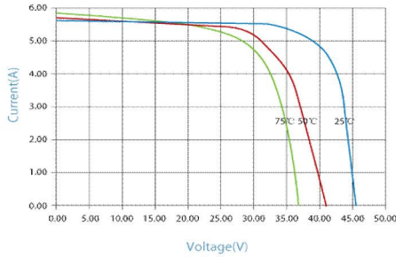
IV-CURVES of PV module RD180TU-36M
