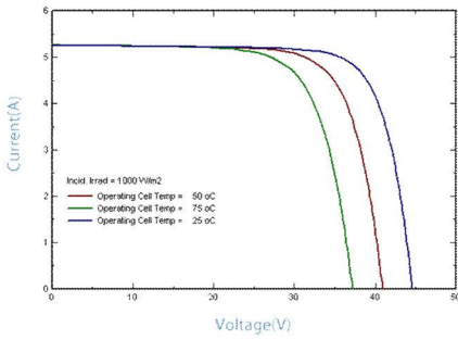
IV-CURVES of PV module RD165TU-36SP
