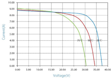
IV-CURVES of PV module RD240TU-30P
