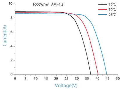
IV-CURVES of PV module RD280TU-36P
