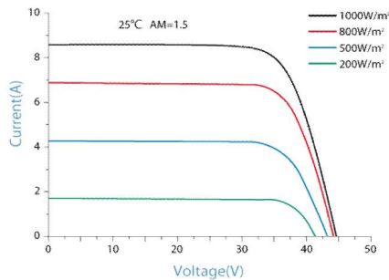
IV-CURVES of PV module RD280TU-36P
