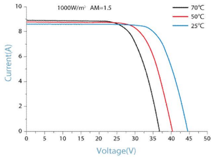
IV-CURVES of PV module RD300TU-36P
