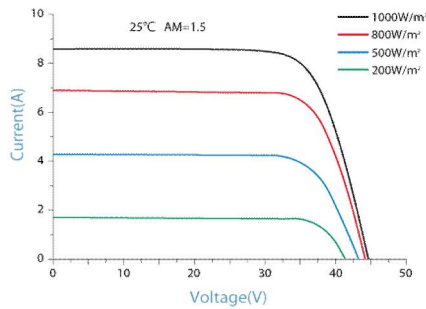
IV-CURVES of PV module RD300TU-36P
