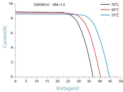
IV-CURVES of PV module RD320TU-36P
