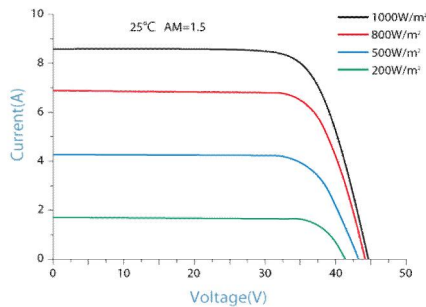
IV-CURVES of PV module RD320TU-36P
